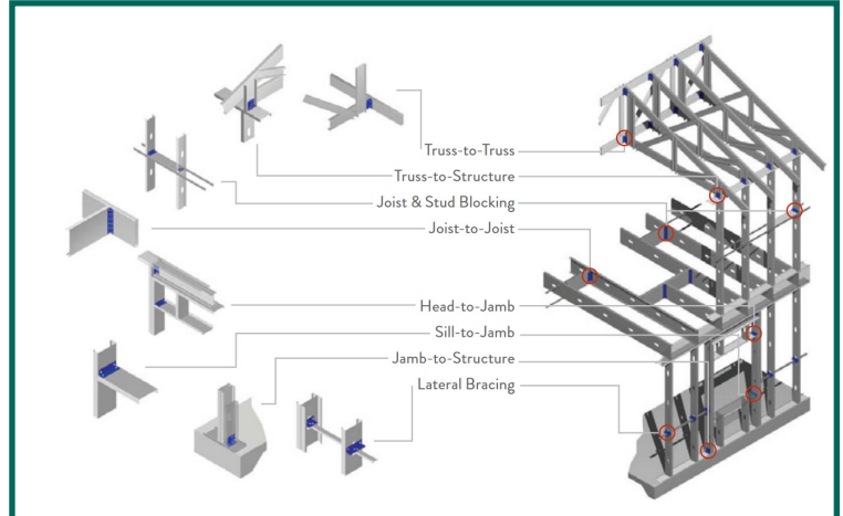
SWIFTCLIP™ 1-1/2" X 3" (LE-SERIES) Installation
