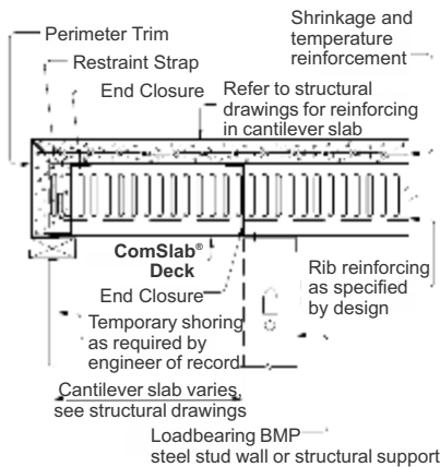
END CANTILEVER DETAIL
