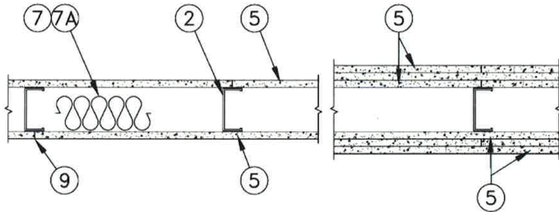
Bearing Wall
