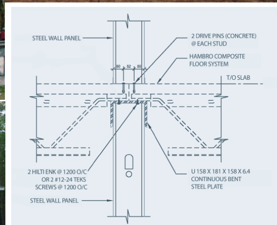
LOAD DISTRIBUTION CHANNEL - DETAIL (ASPEN HEIGHTS CONDOMINIUMS)
